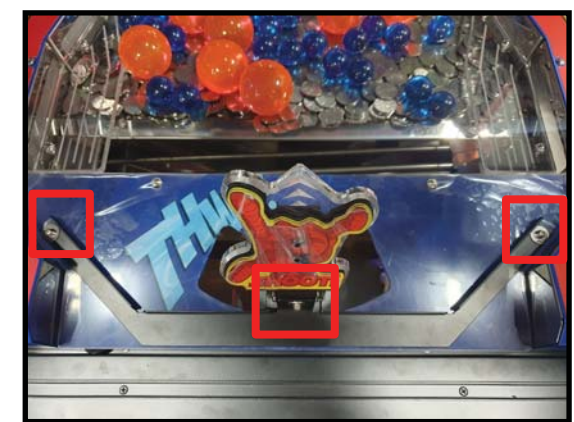
[ 1 ~ 2P ] SHOOTER ASS'Y PACKING BKT_2EA - Bolt, 6 Points *Replace with the supplied TH[M4x10L, 6EA] bolt.
