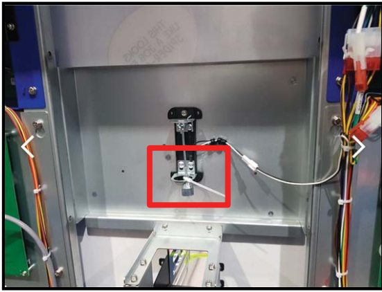
Open the REAR upper door and remove the tie from the TILT ASS'Y_1EA
